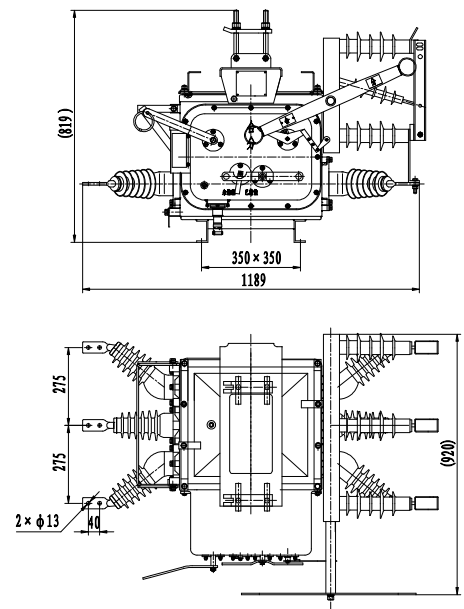
ZW20B-12G Outline and installation dimensions drawing
