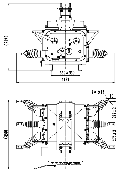
ZW20B-12 Outline and installation dimensions drawing
