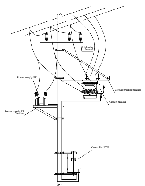
Single-pole lift-mounted installation diagram of circuit breaker
