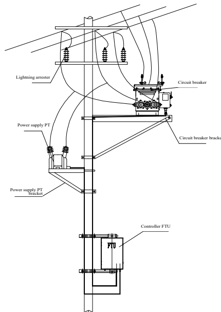
Single-pole seat-mounted installation diagram of circuit breaker
